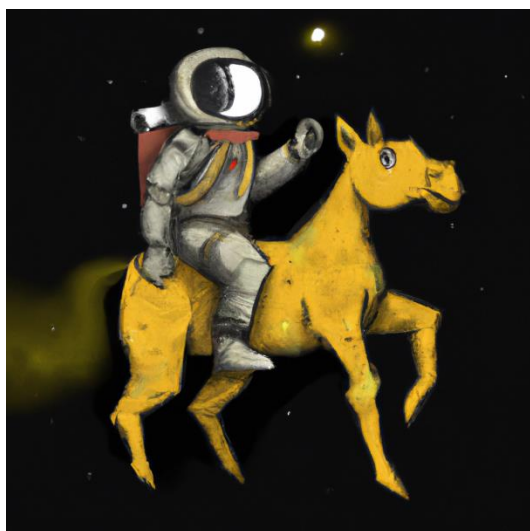
Dall-e-2
